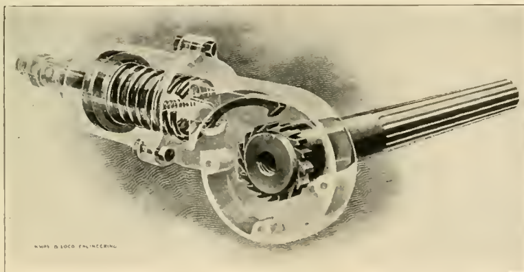
FIG. 2. OPERATION OF THE PAWL AND RATCHET.
